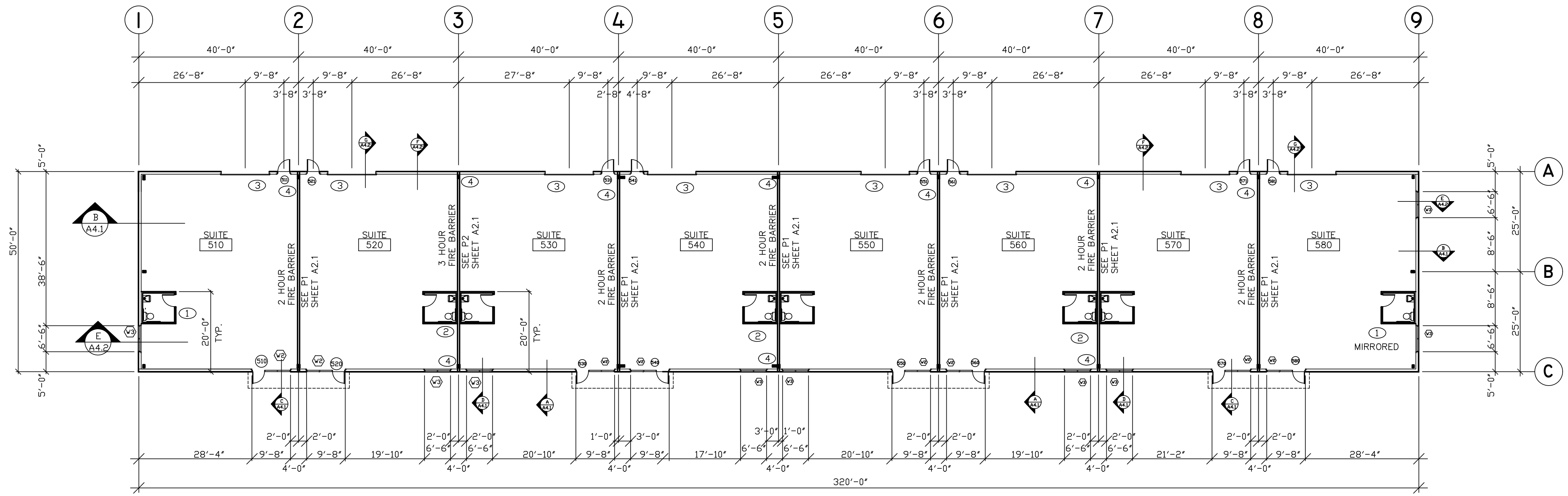
B BUILDING "500" A1.1 1/16" = 1'-0" NORTH
