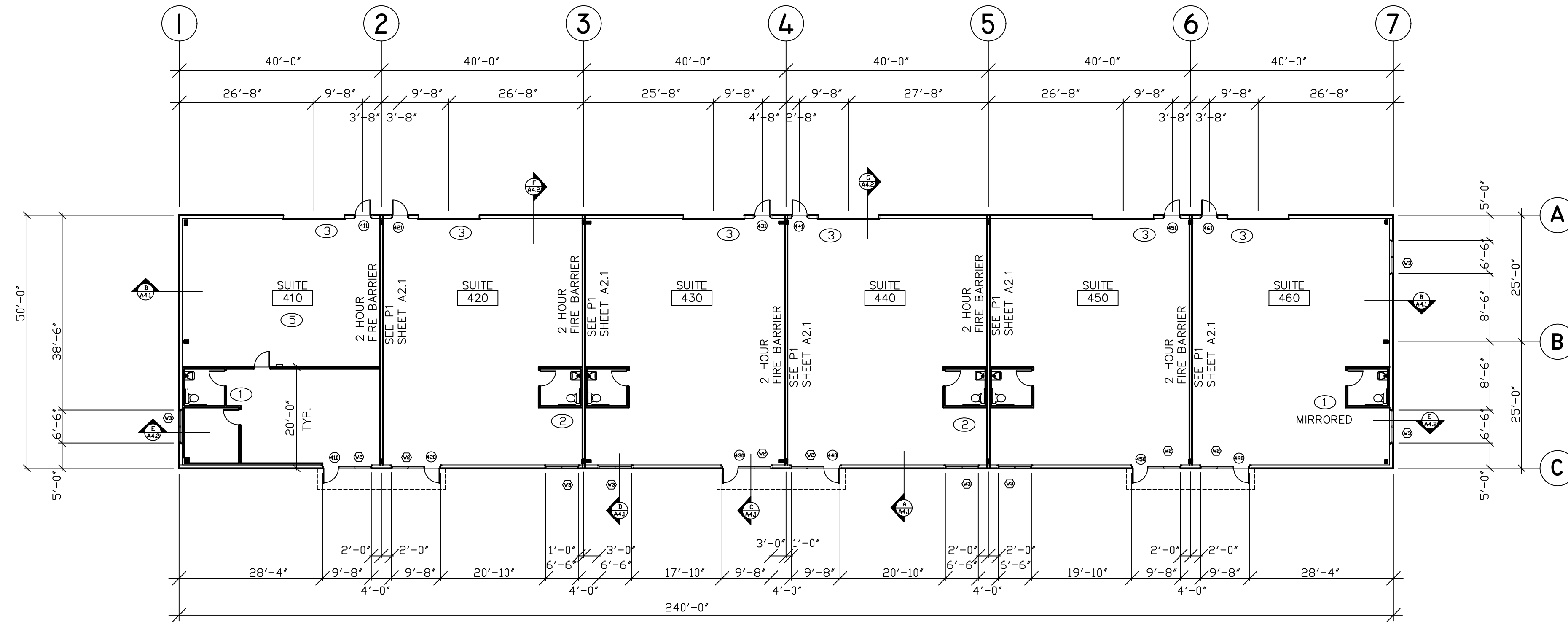
A BUILDING "400" A1.1 1/16" = 1'-0" NORTH
