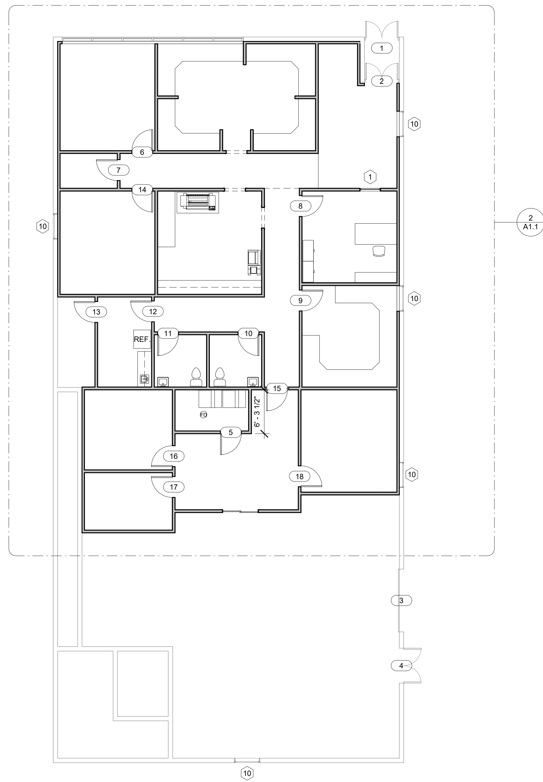
1 Floor Plan 1/8" = 1'-0"
