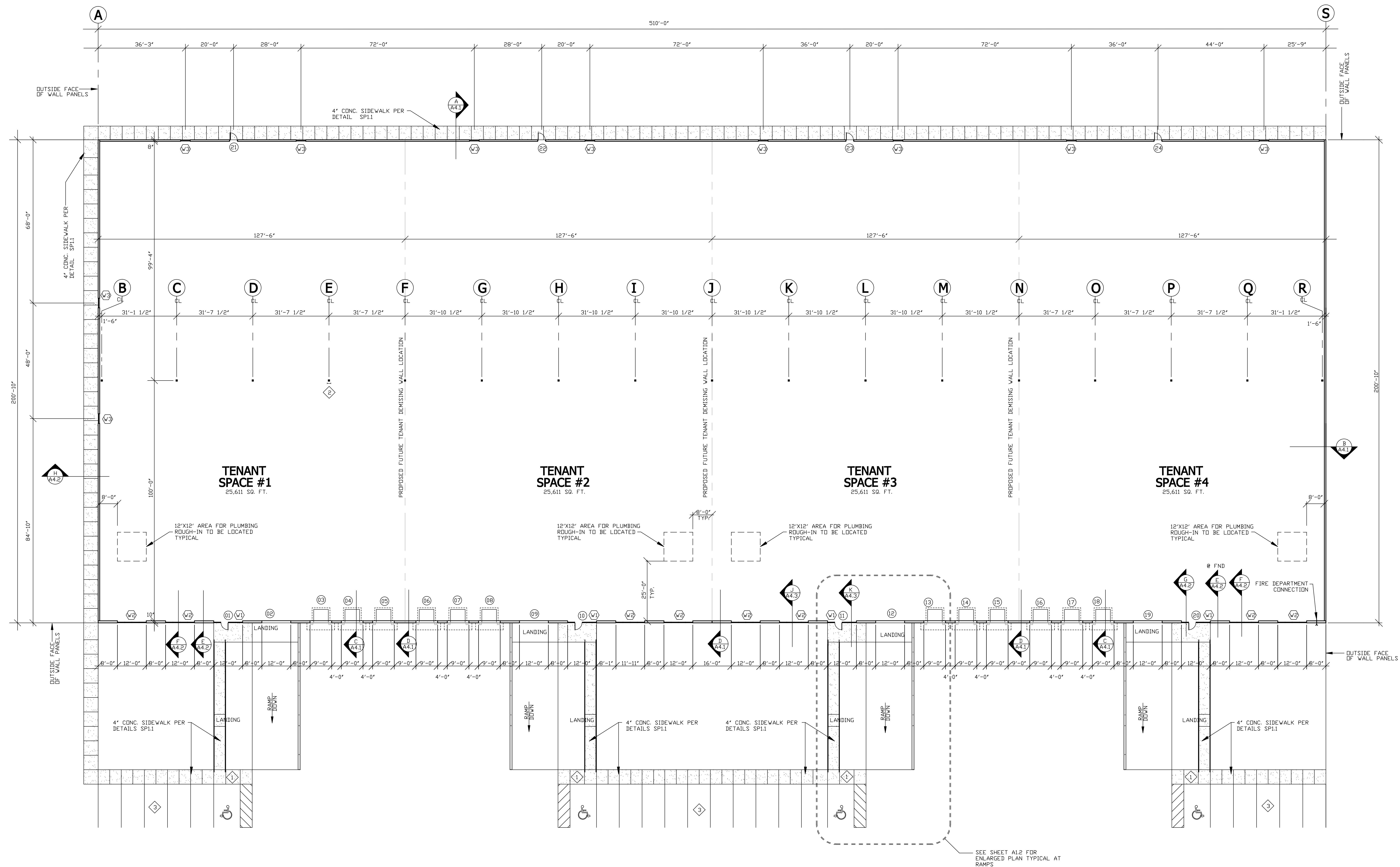
FLOOR PLAN 1/16" = 1'-0" 102,444 SQ. FT.
